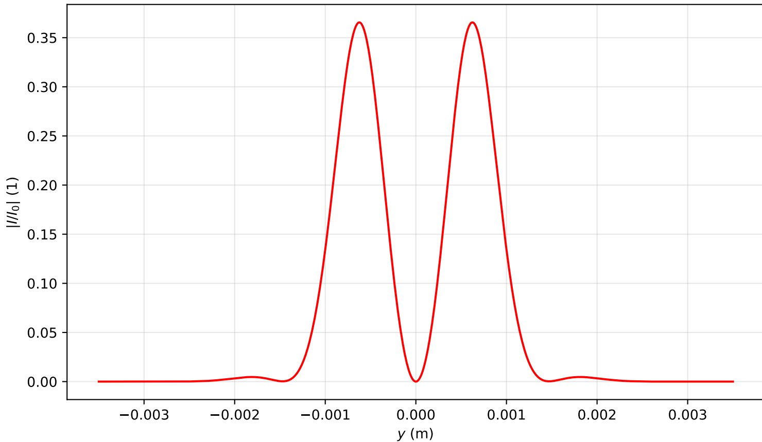
Intensity profile I(x=0, y, z=1.751)/I_0 , P_{in}=4.0P_{cr} , artificial time
